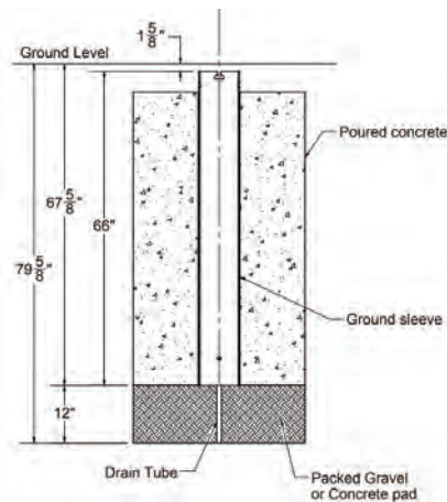
GROUND SLEEVE
