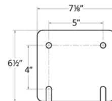
Mounting Plate
