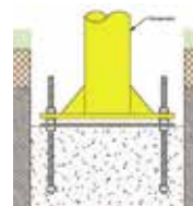
Leveling Plate
