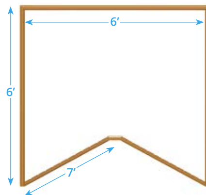
Official Field Lacrosse Goal
