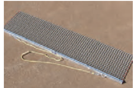
Rigid Drag Mat Rugged steel drag mats with 1inch x 1inch mesh. Mesh is rotated 90° to make mat rigid. Includes heavy duty angle iron and a rope and handle for pulling. Sizes: 4' wide x 18" Length 6' wide x 18" Length
