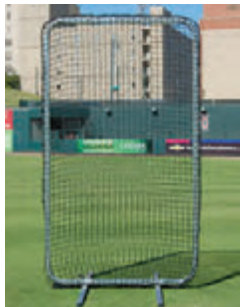
BSQ4274 Proface™ Mini Fungo Screen Heavy-duty 2" square galvanized steel frame. Swaged joints for easy assembly. Detachable push-button legs for easy storage. Heavy duty pillowcase style 2.5 mm #42 netting. Size: 7' x 4'.
