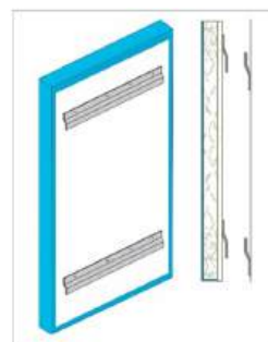
4-Piece Aluminum Z-Channel at Top & Bottom Clean & frameless
