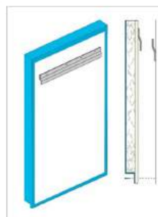
Z-Channel at Top 1" Vinyl Encased Attachment Lip at Bottom Recommended
