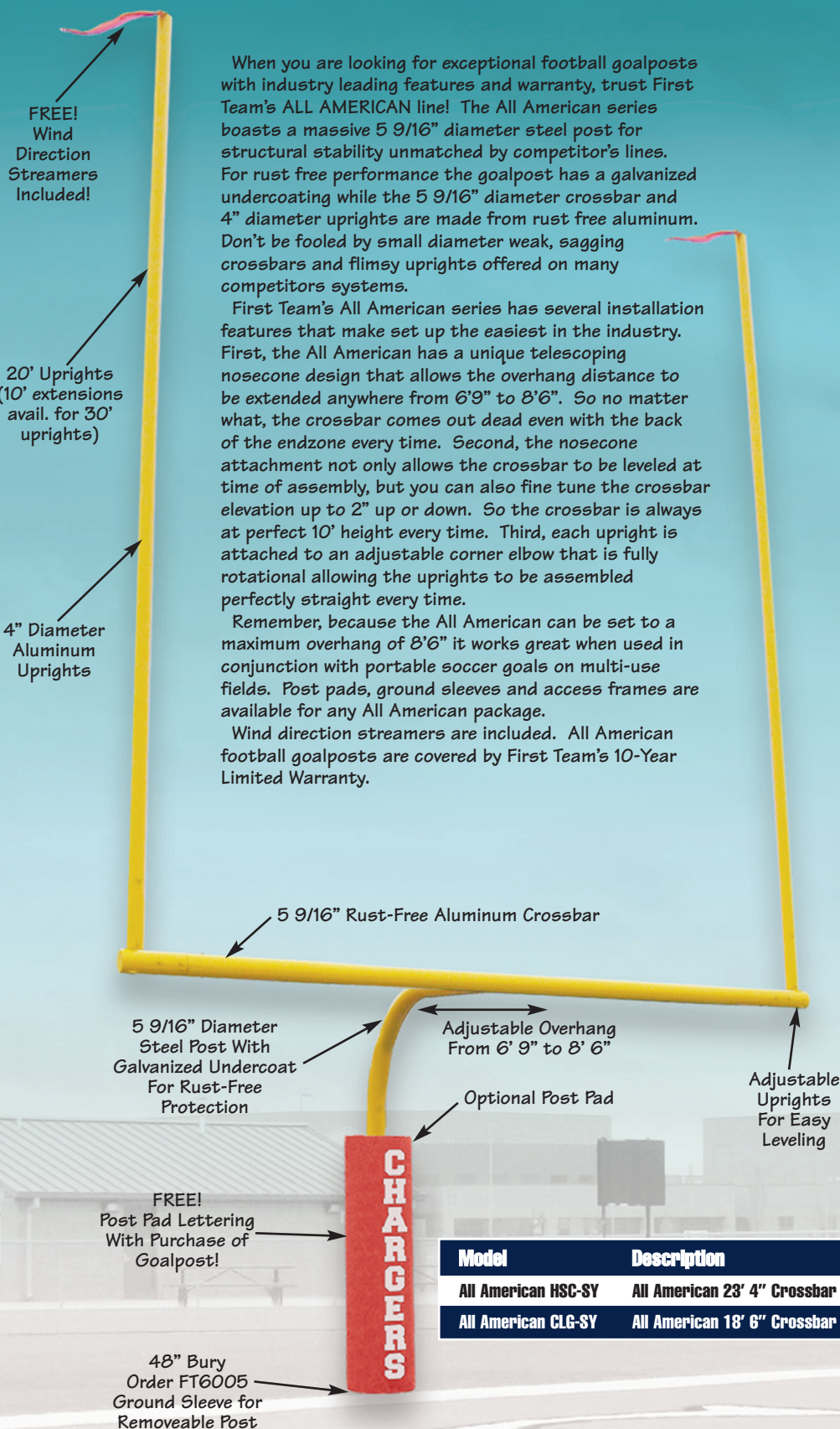
Crossbar & Upright Leveling Feature
