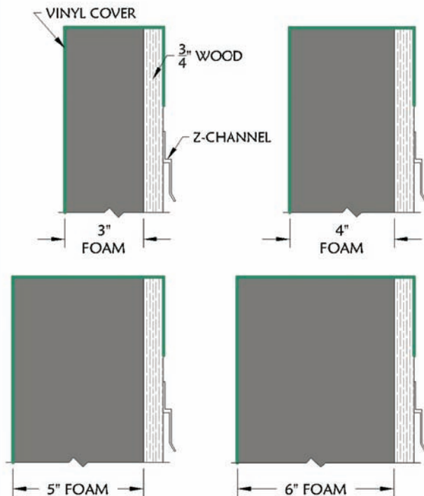
FIELD PAD FOAM THICKNESS OPTIONS (CROSS SECTION OF FIELD PAD SHOWN)
