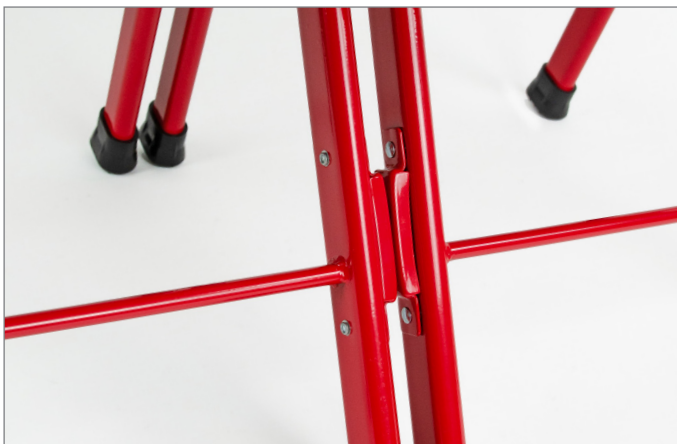
MODEL #DSL-FRAMELOCK connection detail
